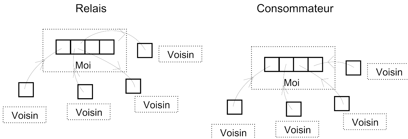
Illustration 26: Anonymat : Relayer versus consommer
